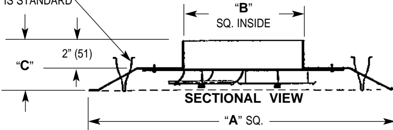
DIMENSIONS LISTED IN INCHES (Millimeters)
