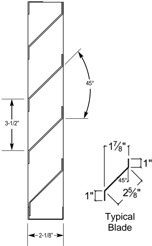
Section View
