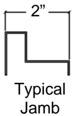
Section View
