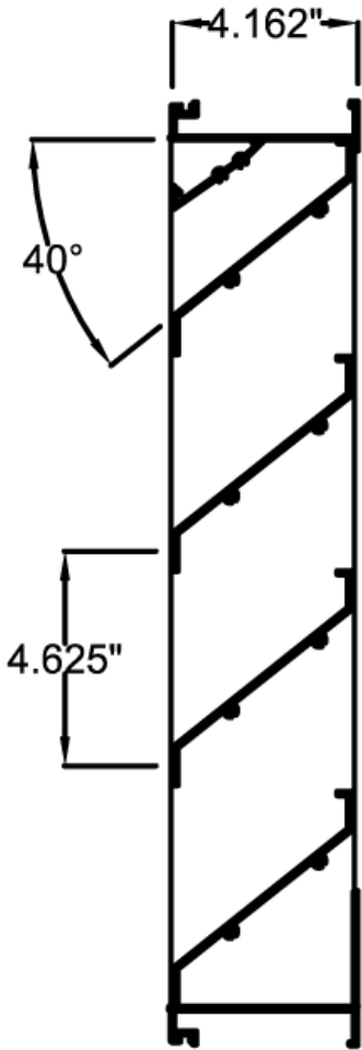
Section View
