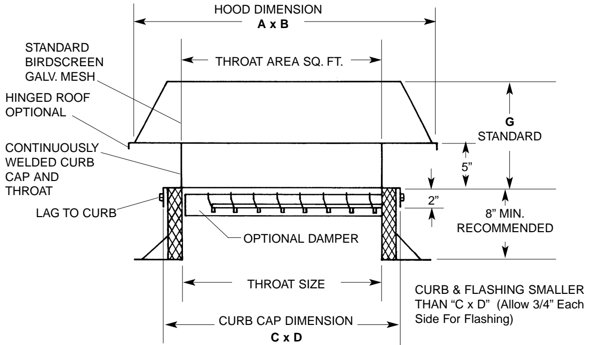
DIMENSIONS LISTED IN INCHES
