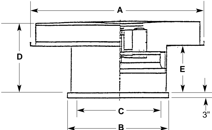
MODEL LTBA: BELT DRIVE (Hoods on 42" - 60" KD) (2) Specify assembled if required
