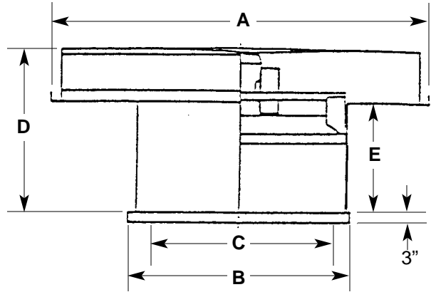
MODEL LTDA: DIRECT DRIVE (Hoods on 42" - 60" KD) (2) Specify assembled if required
