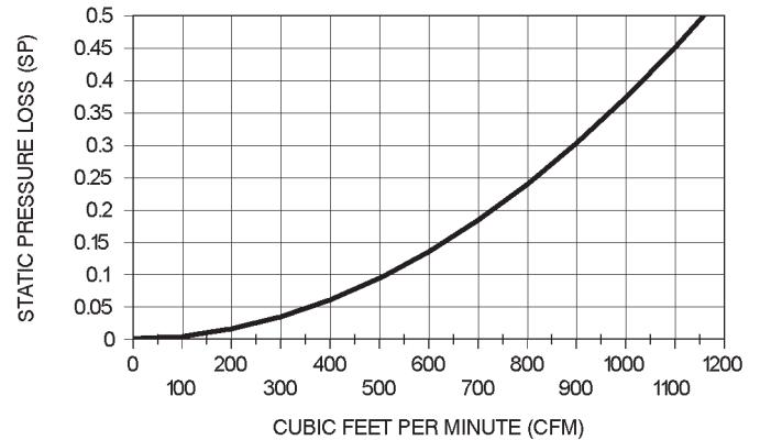
VXCAF12 & VXCAC12 AIRFLOW PERFORMANCE
