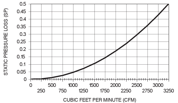
VXCAF20 & VXCAC20 AIRFLOW PERFORMANCE
