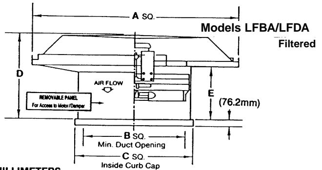
DIMENSIONS LISTED IN MILLIMETERS
