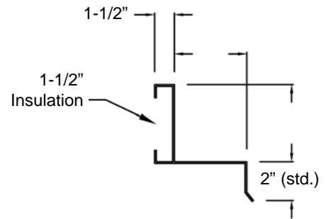
JCAA SECTION
